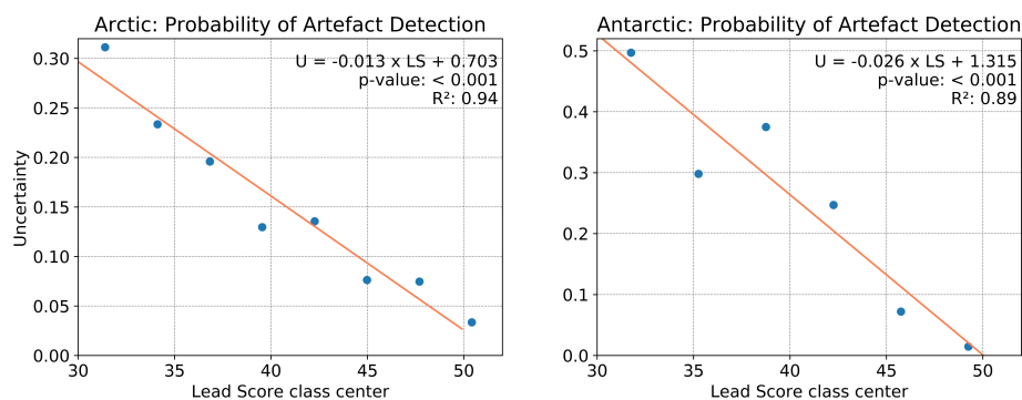
Figure 8. Transfer function for the center Arctic (left) and Antarctic (right) based on which a pixel-wise uncertainty is calculated for all potential sea ice leads. The respective coefficients for the functions are given in the graphic.
